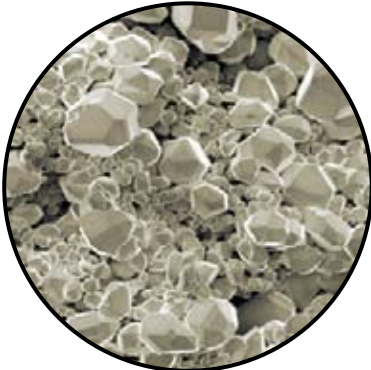
Photo 1B: A battery plate covered in heavy sulfation buildup. This buildup acts as an insulation barrier and reduces the battery’s ability to accept and release energy.
